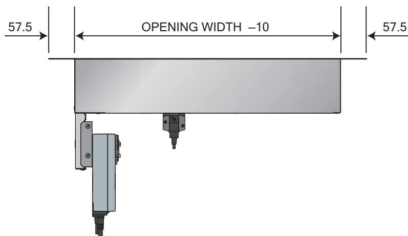
View from actuator side (non-access side)
